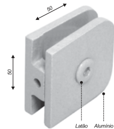
Suporte central 50x50mm
