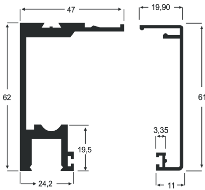
AP - 1 1,193 Kg/m
