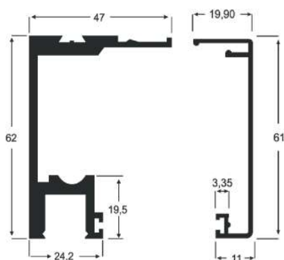
AP - 1 1,193 Kg/m
