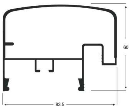
AP - 83 1,186 Kg/m
